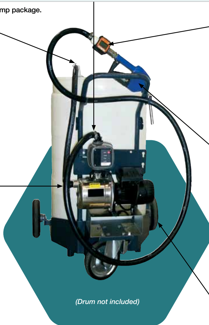
FLTBEN113EA 1/3 HP Manual Start Centrifugal Pump
